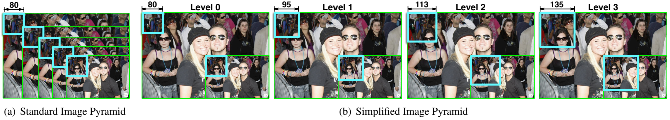
Figure 6. Comparison between the standard image pyramid and the simplified image pyramid we adopted: across the levels of the simplified image pyramid, base face size varies but feature descriptors are shared to save computational resource.
