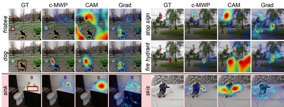
Fig. 5. Example attention maps using GoogleNet. For visualization, the maps are superimposed on the images after some postprocessing (slight blur for Grad and thresholding for CAM). ( Top two rows ) Our c-MWP is very discriminative and can often localize challengingly small objects like frisbee , stop sign and fire hydrant . ( Bottom row ) Two typical failure cases of top-down neural attention are shown. Since faucet often co-occurs with sink , the CNN’s attention falsely focuses on the faucet in the image. It is the same case for ski poles and skis .
