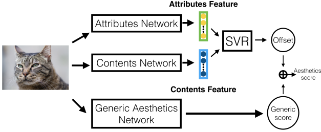
Figure 3: An overview of the proposed residual-based personalized aesthetics model.
