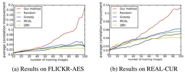
Figure 6: Evaluation of active learning approaches on (a) FLICKR-AES and (b) REAL-CUR on unseen images in the photo album.
