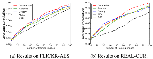
Figure 5: Evaluation of active learning approaches on (a) FLICKR-AES and (b) REAL-CUR on all the images in the photo album.
